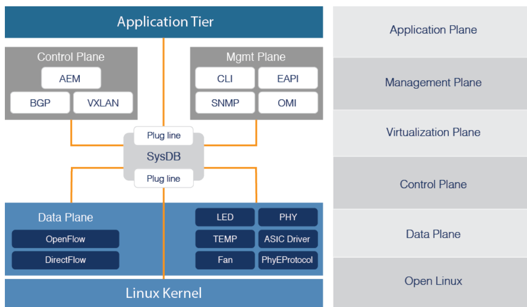
Figure 7: EOS Architecture
