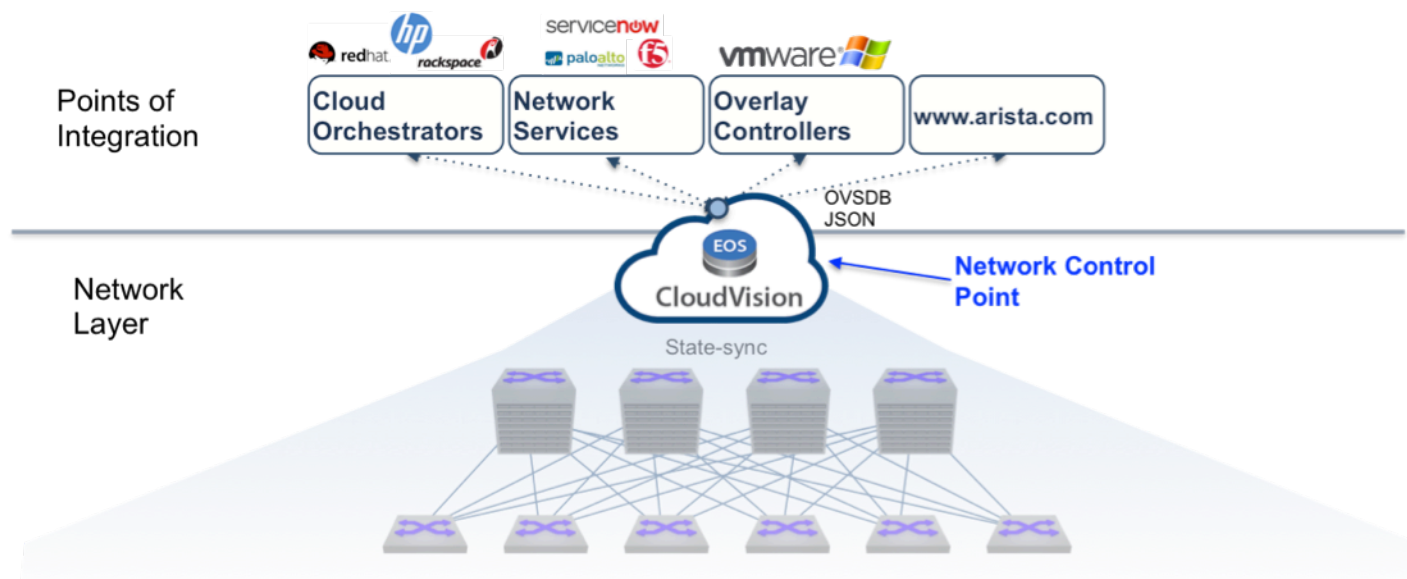
Figure 8: EOS CloudVision
